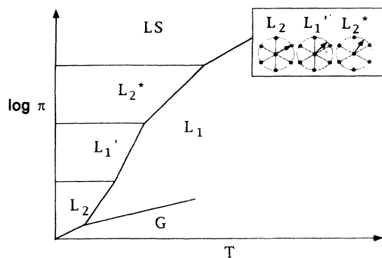
FIG. 1. Schematic pressure-temperature ( \pi - T ) phase diagram showing several of the monolayer phases that have been identified in fatty acids and their esters. The relative locations of the gas ( G ), liquid-expanded ( L_1 ), and superliquid phases ( LS ) are much the same for many substances. The locations of the other phases and the positions of the boundaries between them are more variable and less well known. The inset shows the orientation of the molecular tilt azimuth with respect to the local sixfold structure of the head groups that exists in the three tilted hexatic phase L_1' , L_2 , and L_2^* .
